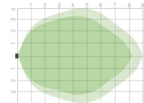
Montaggio a parete (m) Wall mounting (m)
